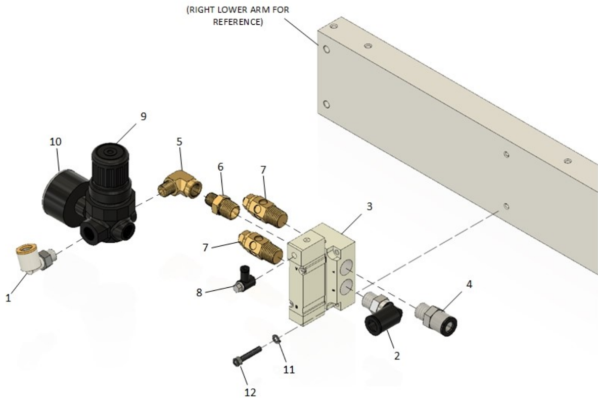
Figure 18: TF01-17 LOWER REGULATOR ASSY
