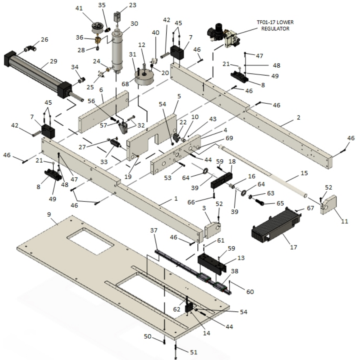
Figure 9: TF01-08 LOWER FRAME ASSY
