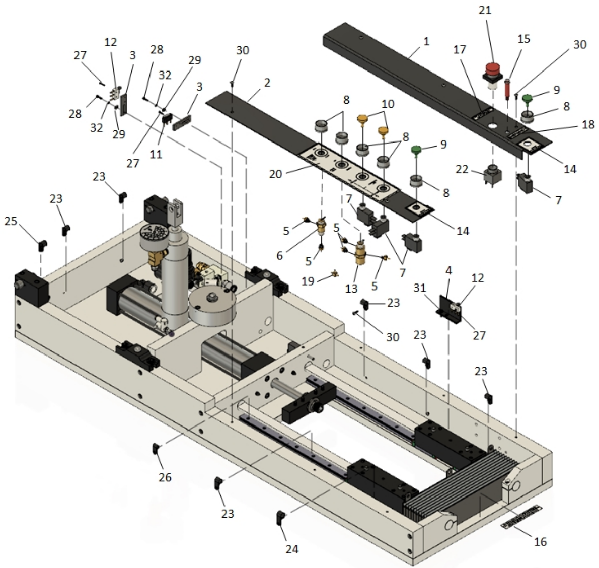
Figure 10: TF01-09 LOWER FRAME ELECTRICAL ASSY
