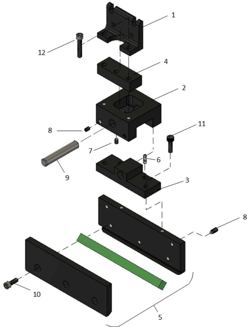
Figure 12: TF01-11 FLOATING SQUEEGEE ASSY
