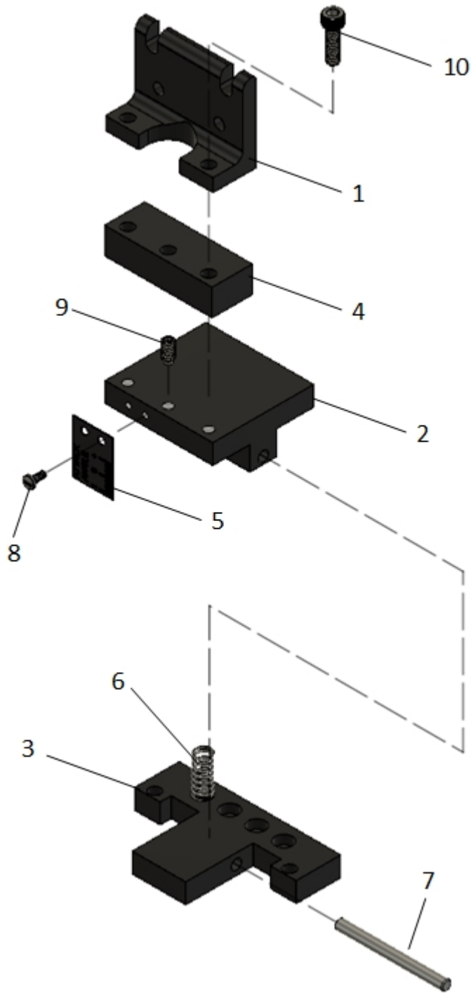
Figure 8: TF01-07 ATTACK ANGLE ASSY
