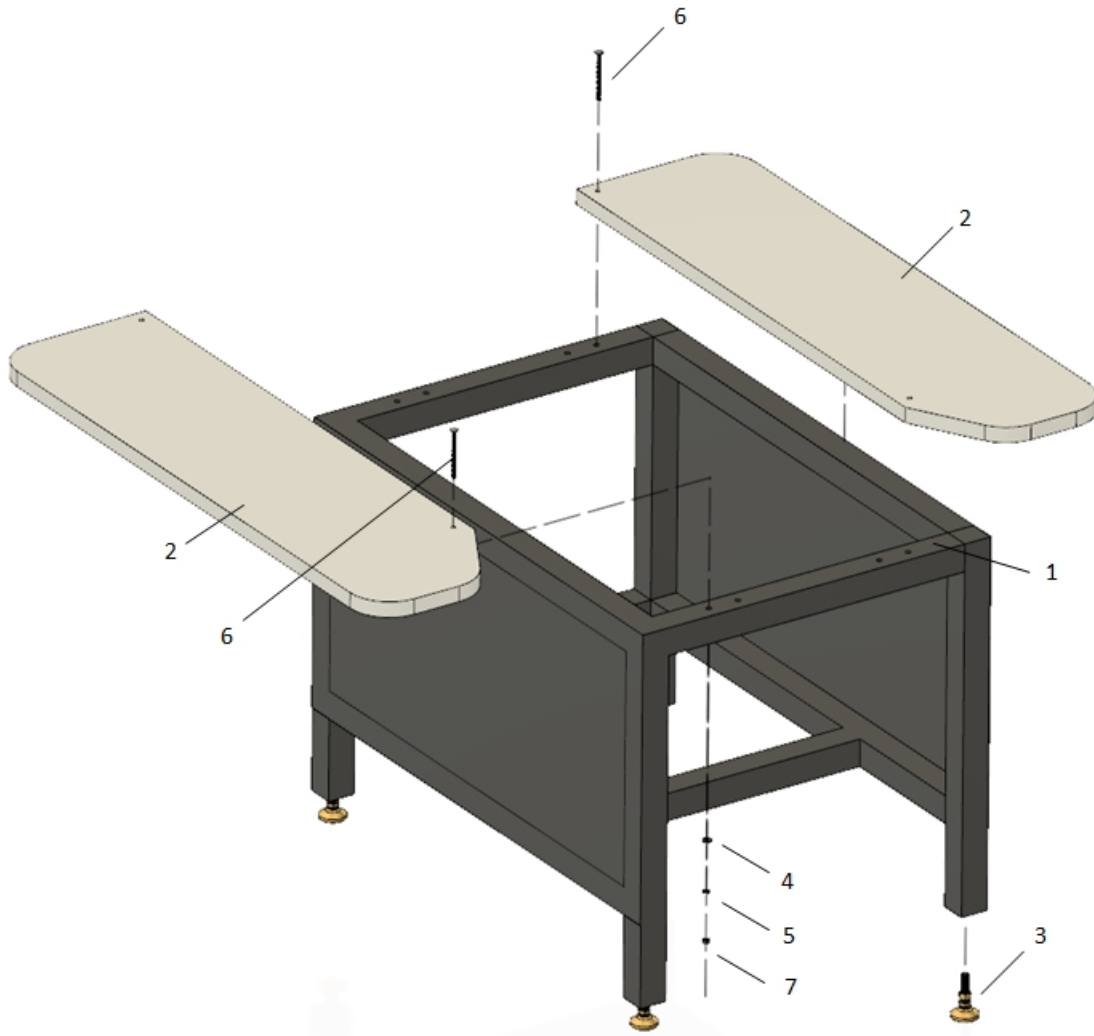
Figure 16: TF01-15 MACHINE BASE ASSY
