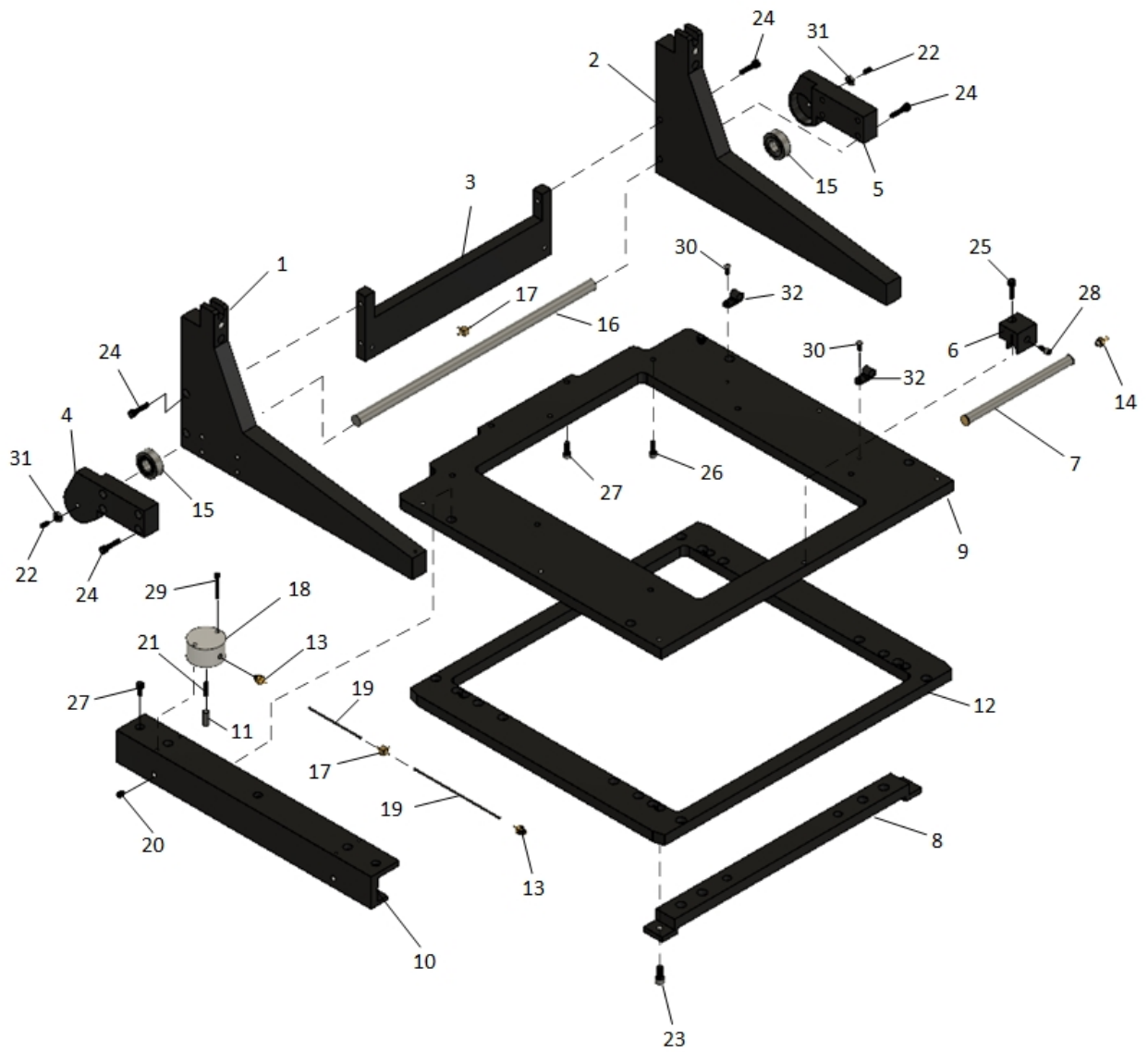
Figure 14: TF01-13 TILT ARM ASSY
