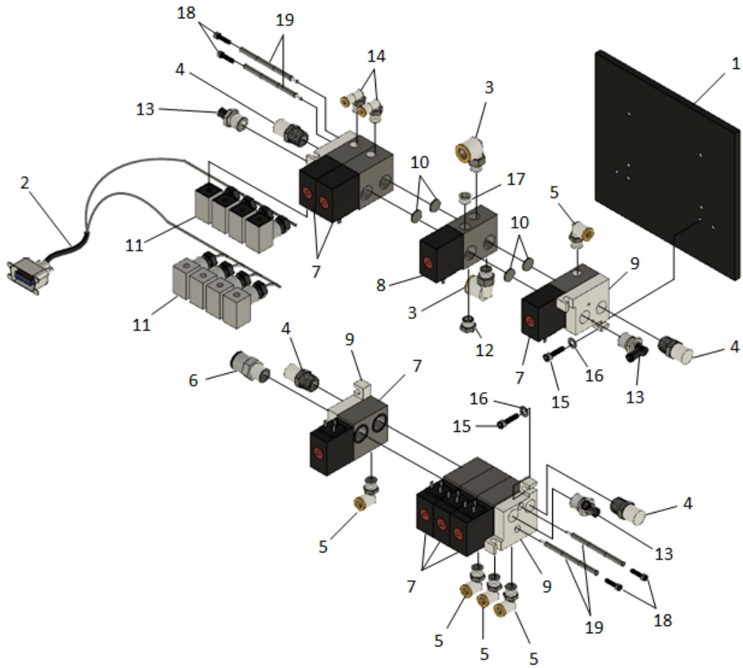
Figure 13: TF01-12 SOLENOID BANK ASSY
