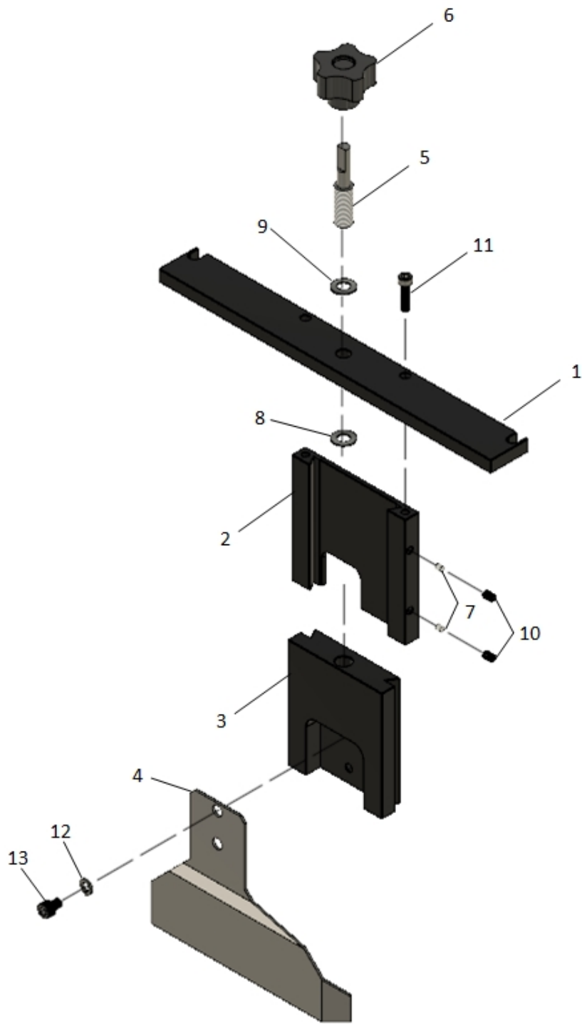
Figure 7: TF01-06 FLOOD BLADE ASSY
