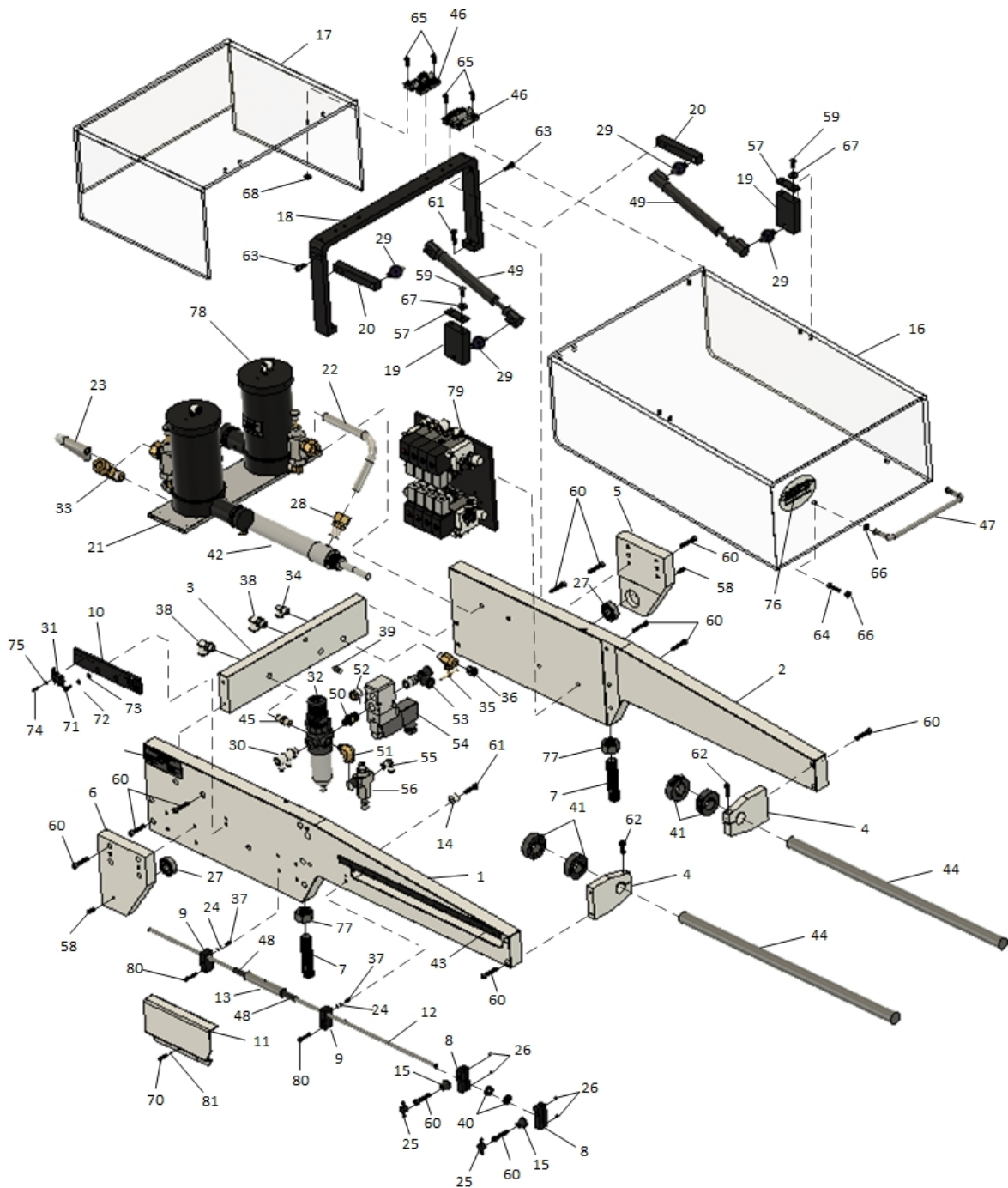
Figure 6: TF01-05 UPPER FRAME ASSY
