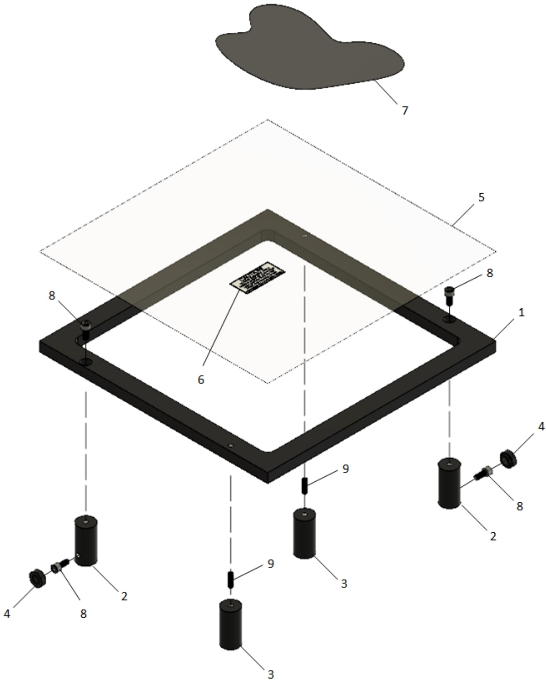
Figure 11: TF01-10 MYLAR FRAME ASSY
