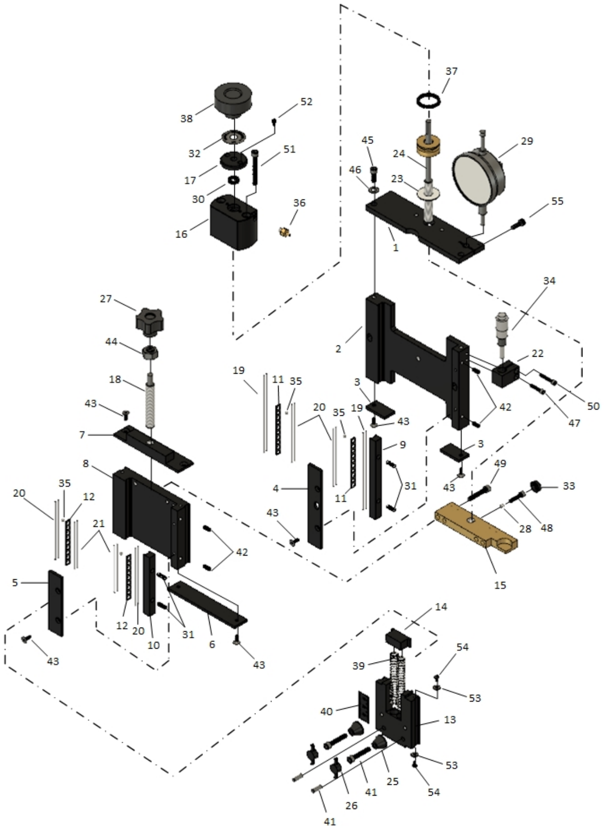
Figure 3: TF01-02 SQUEEGEE ASSY
